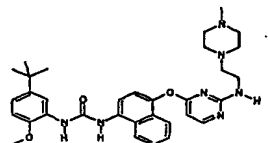
1-(5-tert-Butyl-2-methoxy-phenyl)-3-(4-{2-[2-(4-methylpiperazin-1-yl)ethylamino]-pyrimidin-4-yloxy}-naphthalen-1-yl)-urea;
